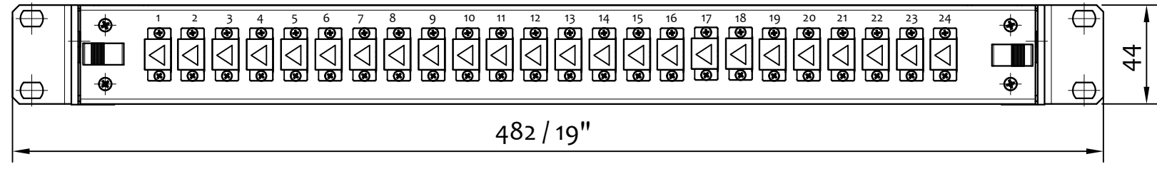
PATCHPANEL 1U - 24x SC/APC FULLY LOADED
