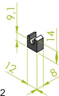
M6 version 1x M6 Thread
