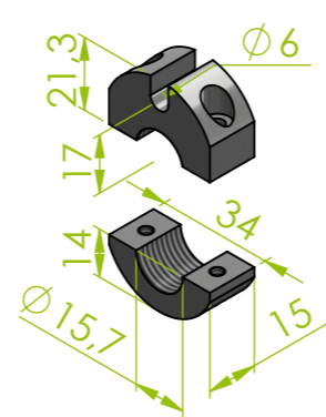
Steel strand version D15,7mm 2xM4
