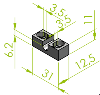
XY version 2xM4 DIN912
