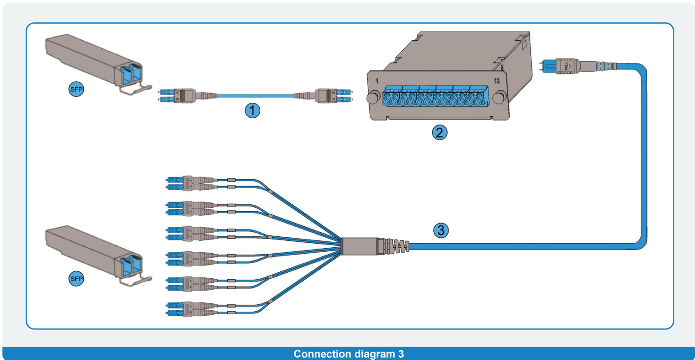
Connection diagram 3
