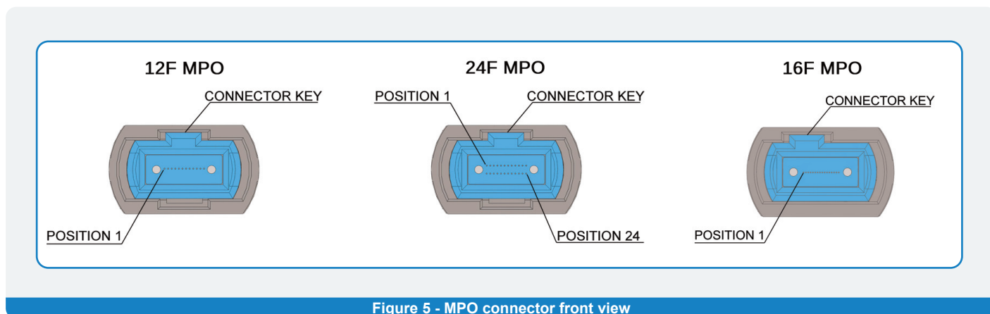
Figure 5 - MPO connector front view
