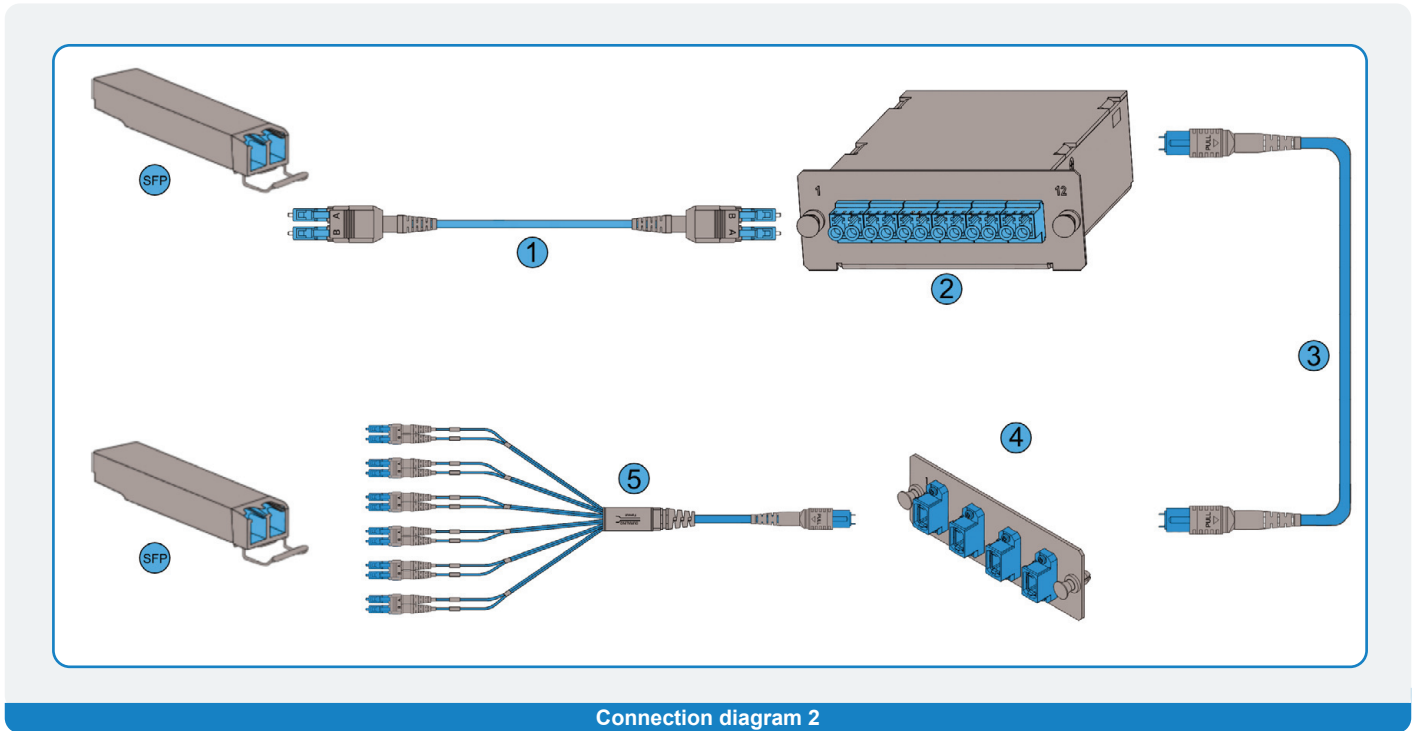
Connection diagram 2
